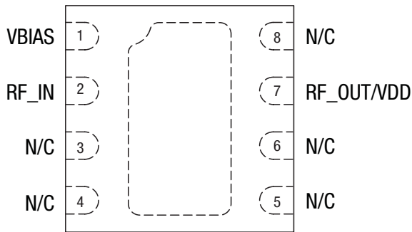
Figure 2. SKY67012-396LF Pinout – 8-Pin DFN (Top View)
